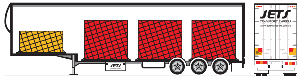
Enclosed trailer configured with 1 lower deck and 3 AQ6 main deck pallets (PMC, M1)
