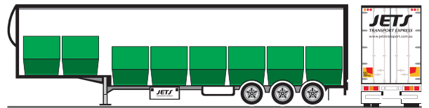
Enclosed trailer configured with 8 AKE (LD-3)
